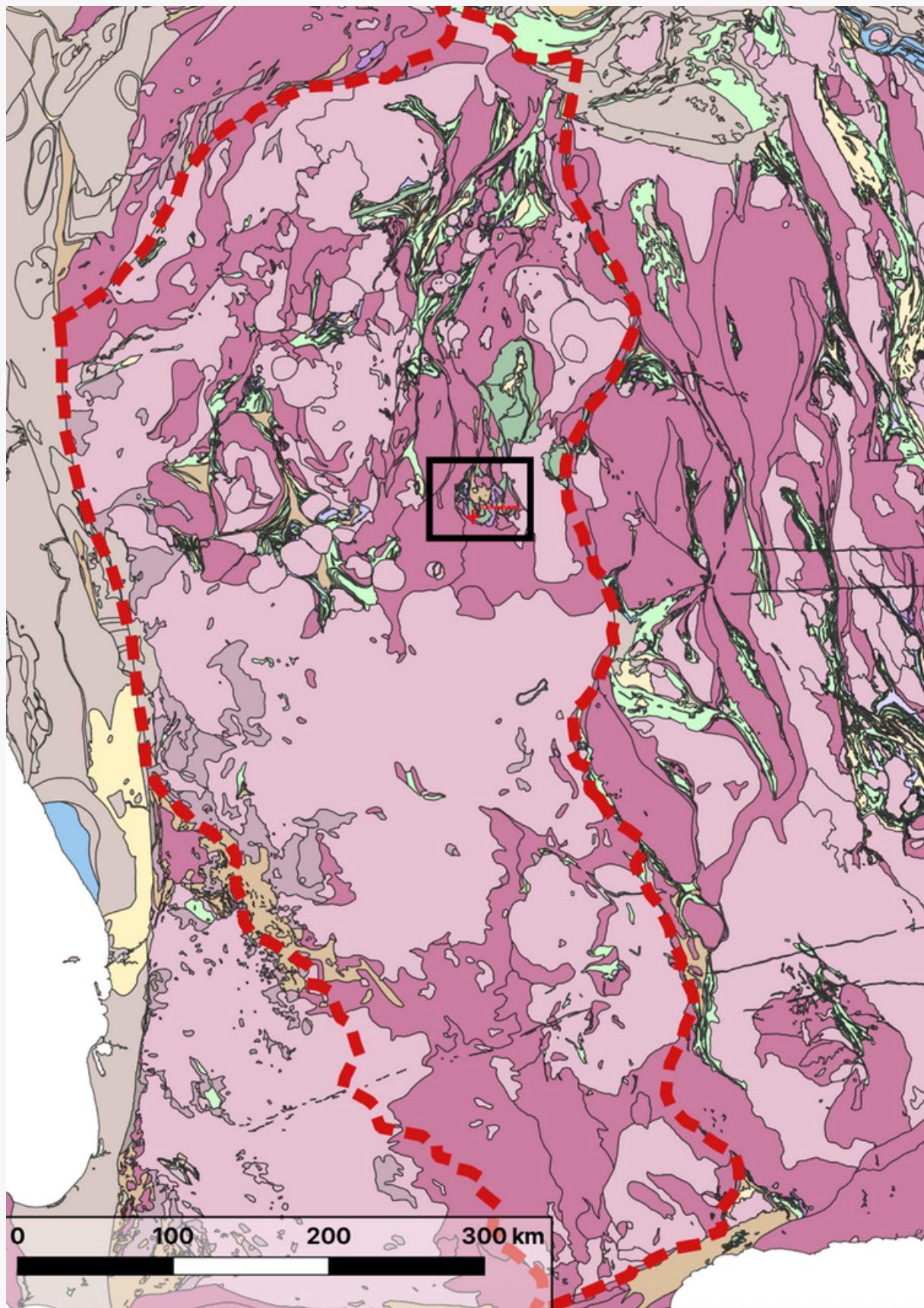
Figure 2 - 1:500,000 interpreted bedrock geology of the Murichson Domain
