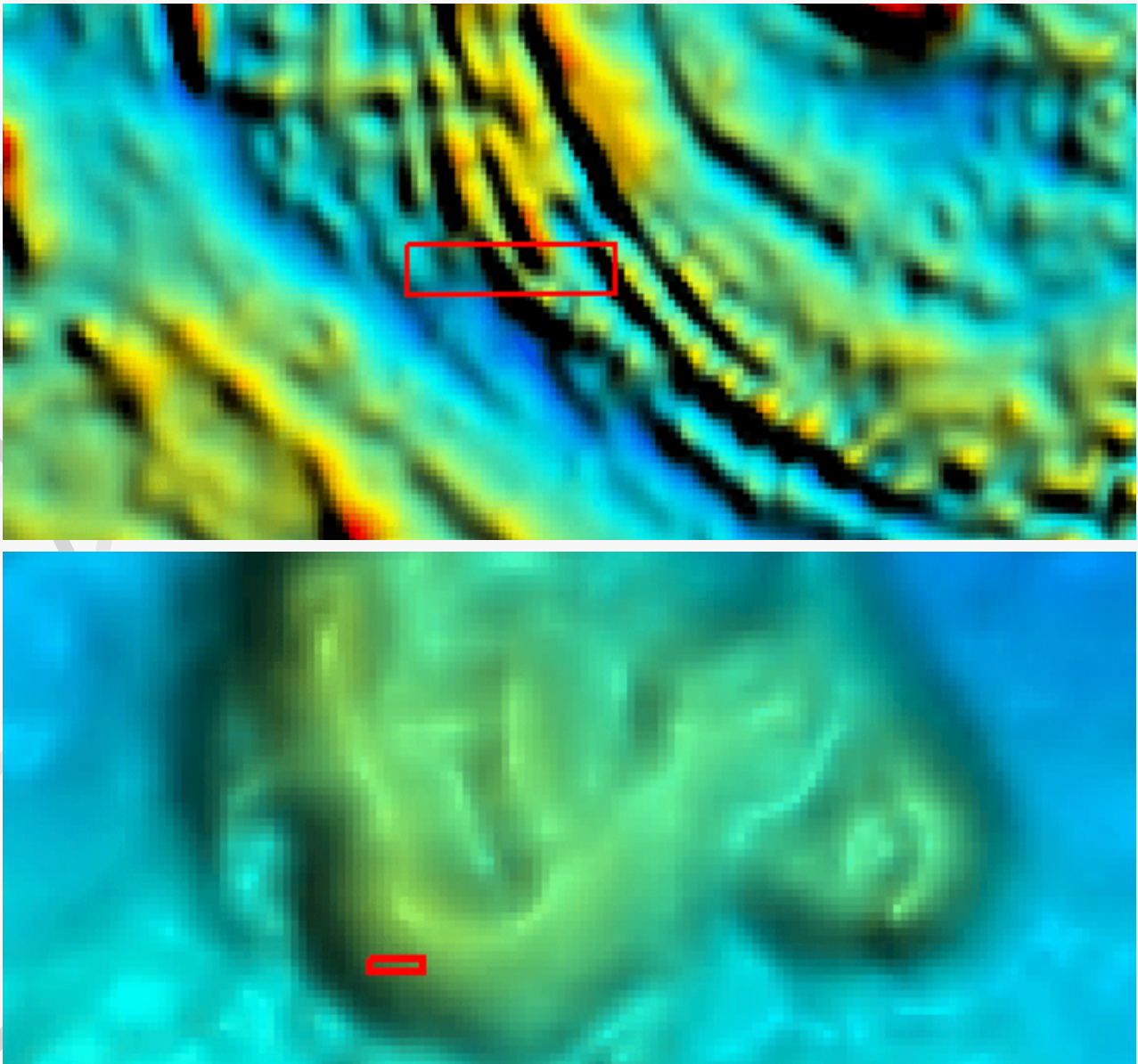
Figure 5- Interpreted GSWA Gravity (top) and Magnetics (bottom) of the tenement
