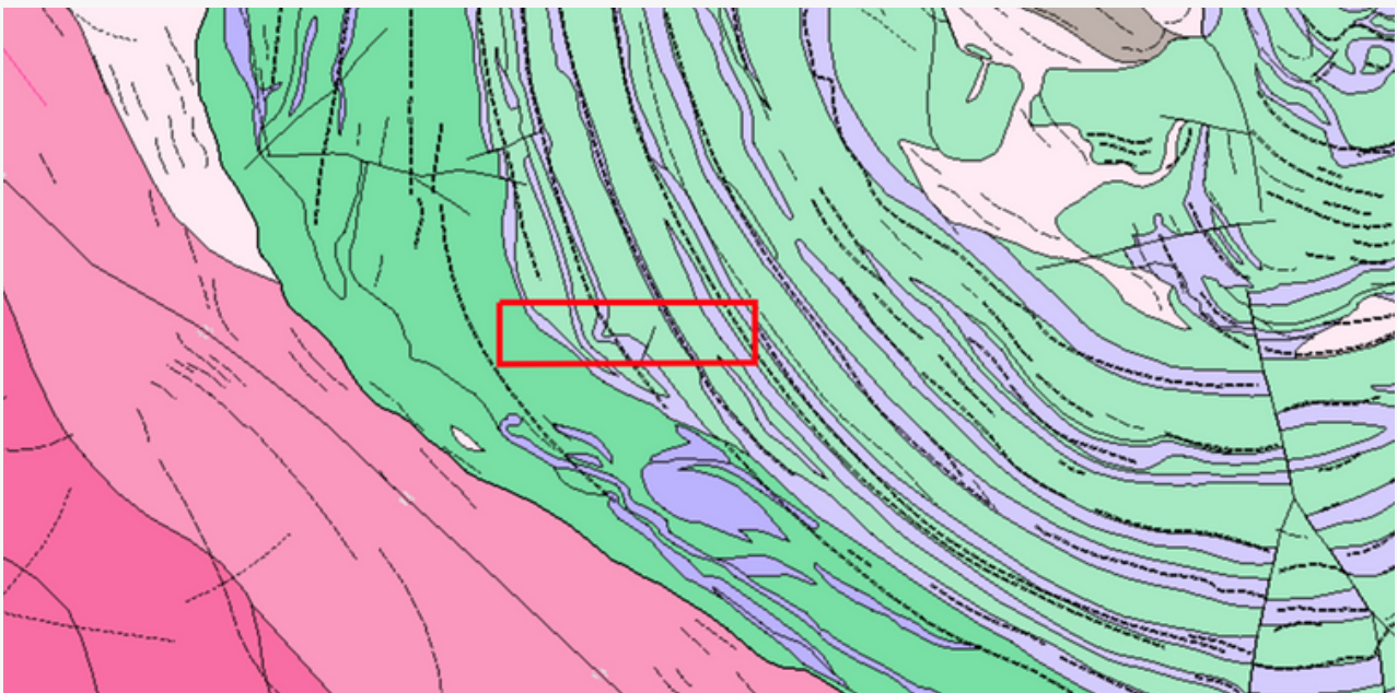
Figure 4- 1:100,000 bedrock geology of P 59/2460.
