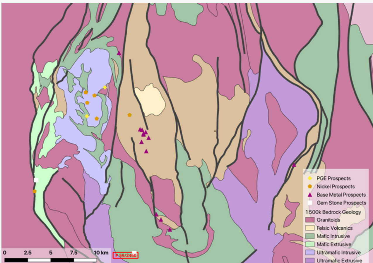
Figure 3 - Tenement draped over 1:500,000 interpreted bedrock geology.
