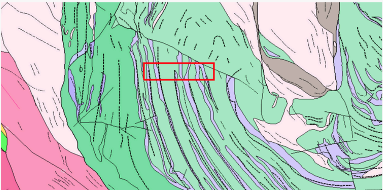
Figure 4- 1:100,000 bedrock geology of P 59/2466.
