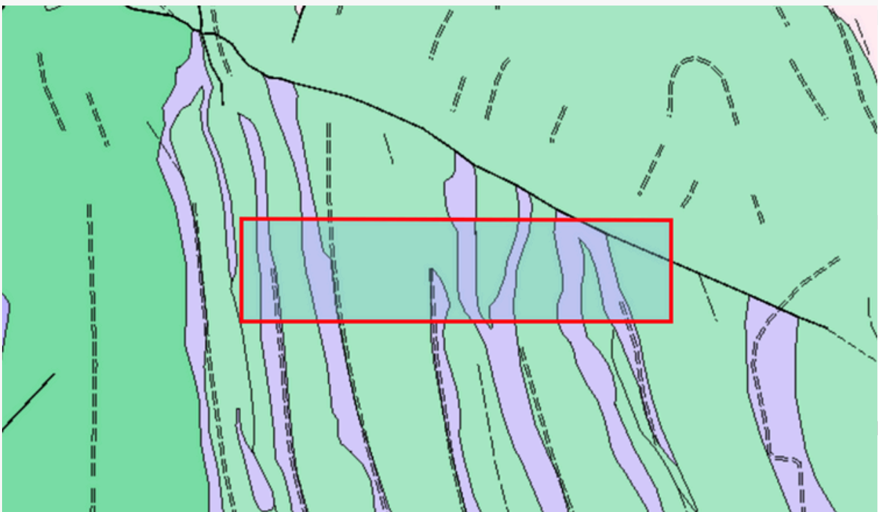
Figure 5- Simplified Geological Mapping
