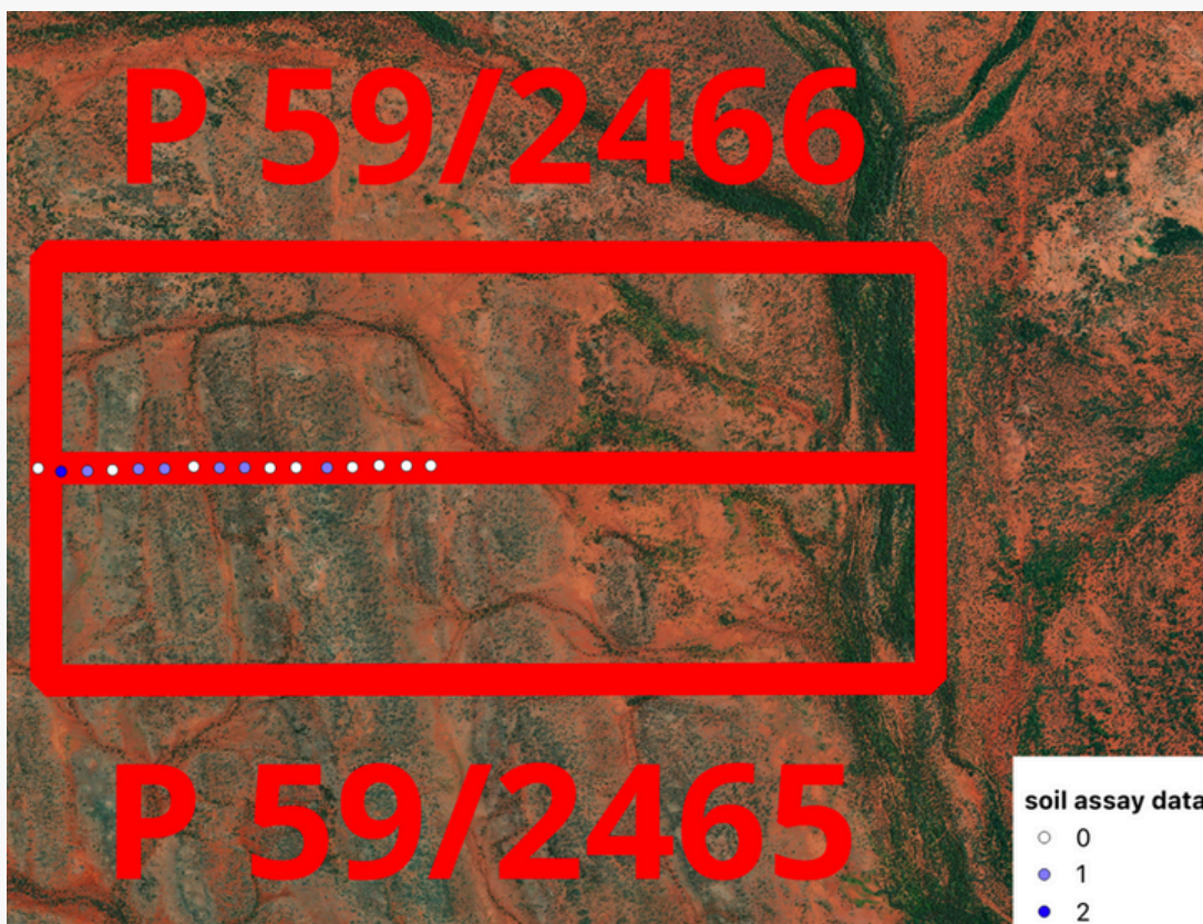
Figure 5- soil sampling data (values in ppb Au)
