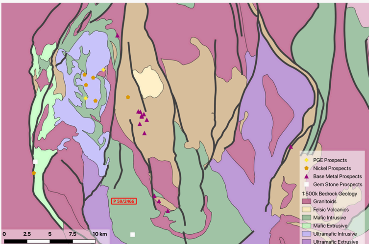
Figure 3 - Tenement draped over 1:500,000 interpreted bedrock geology.
