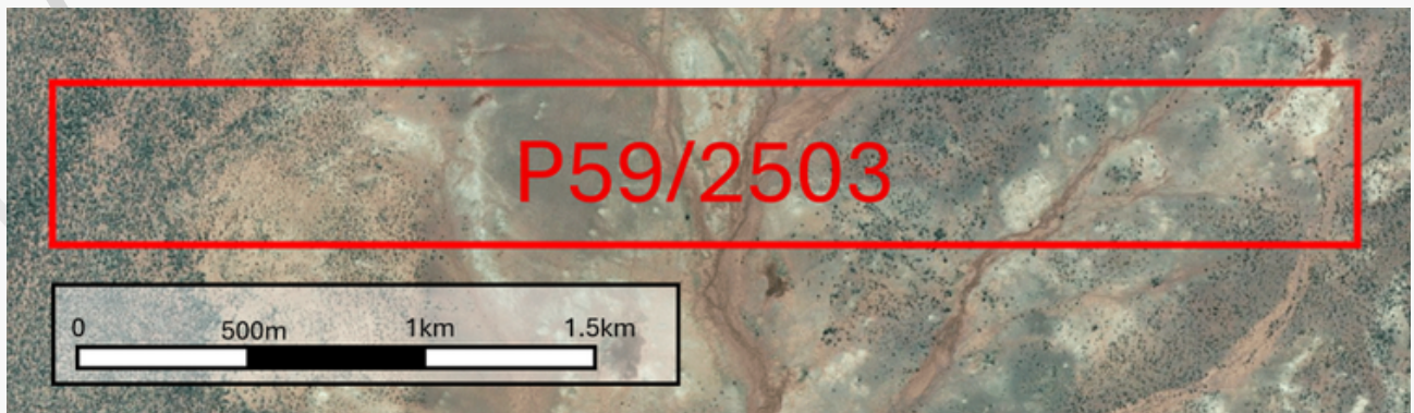
Figure 1 - Project satellite map.
