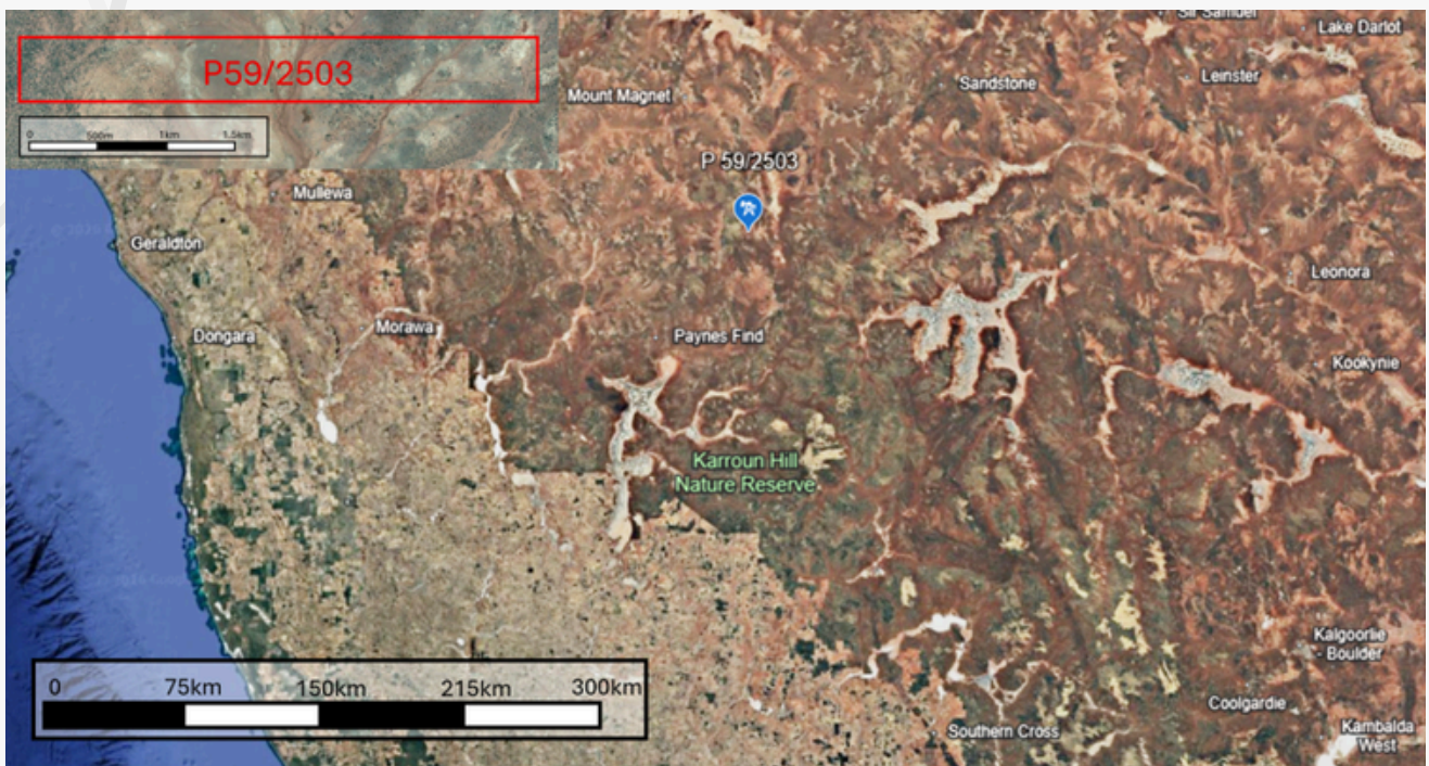
Figure 2 - Project location map.
