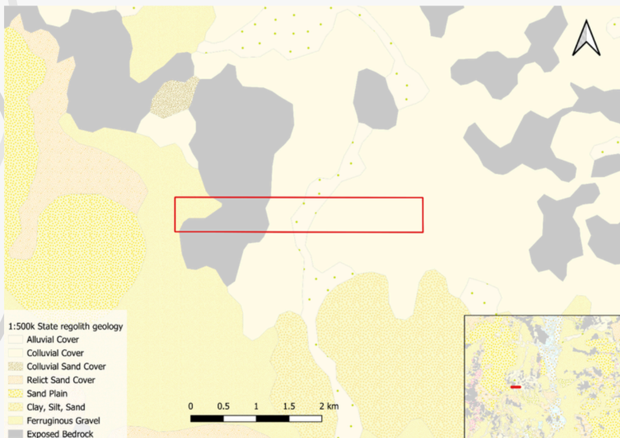
Figure 4 - GSWA 1:500k regolith profile of the project.
