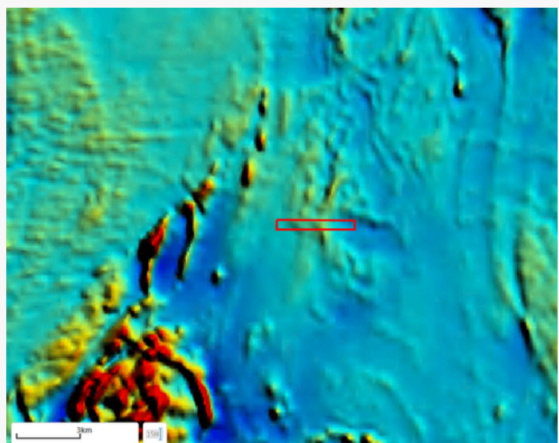
Figure 7- GSWA magnetic anomaly of project
