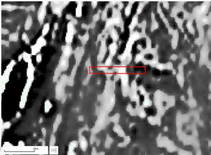
Figure 8- GSWA 1VD magnetic imagery of project
